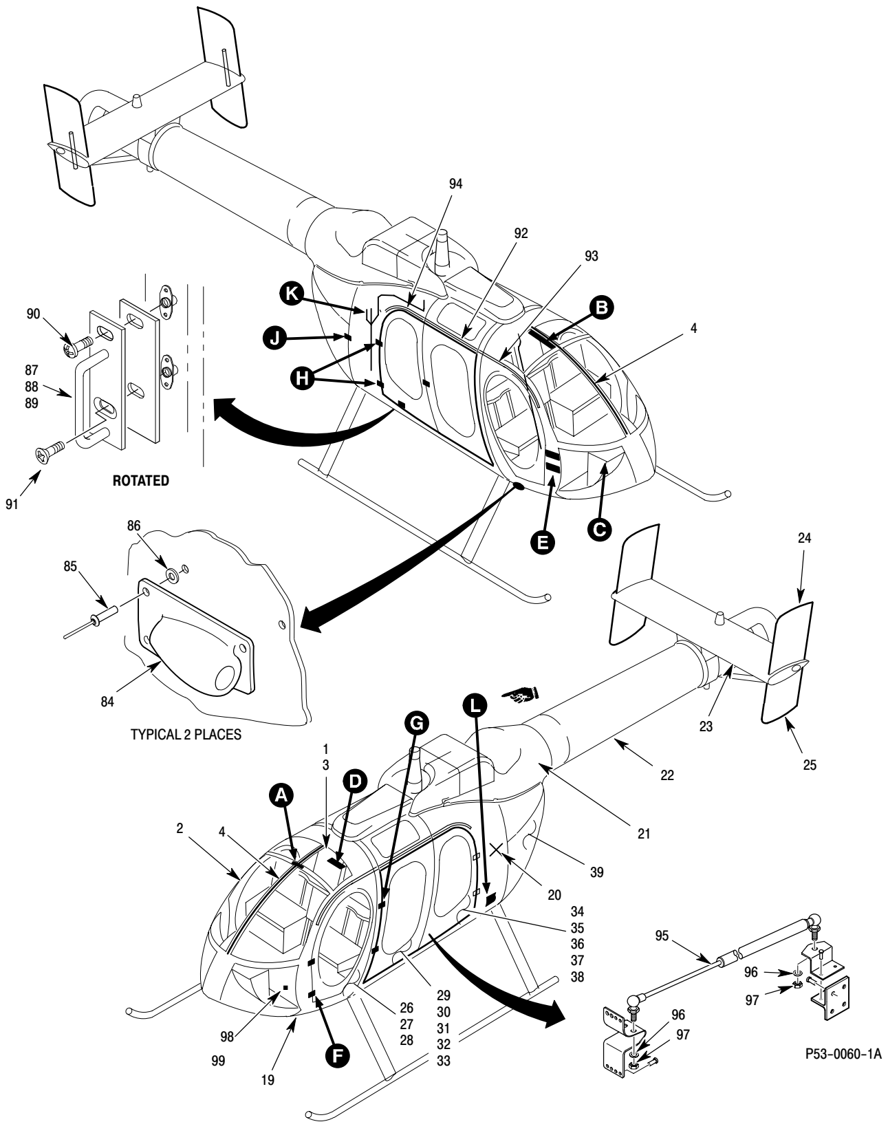
Figure 1. Fuselage Structure Complete - 600N (Sheet 1 of 6)
